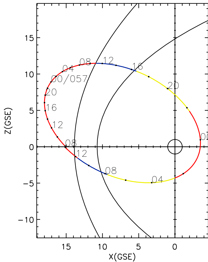
CLUSTER 2 orbit 2022 056 (02/25) 07:51 UT to 2022 058 (02/27) 14:06 UT
