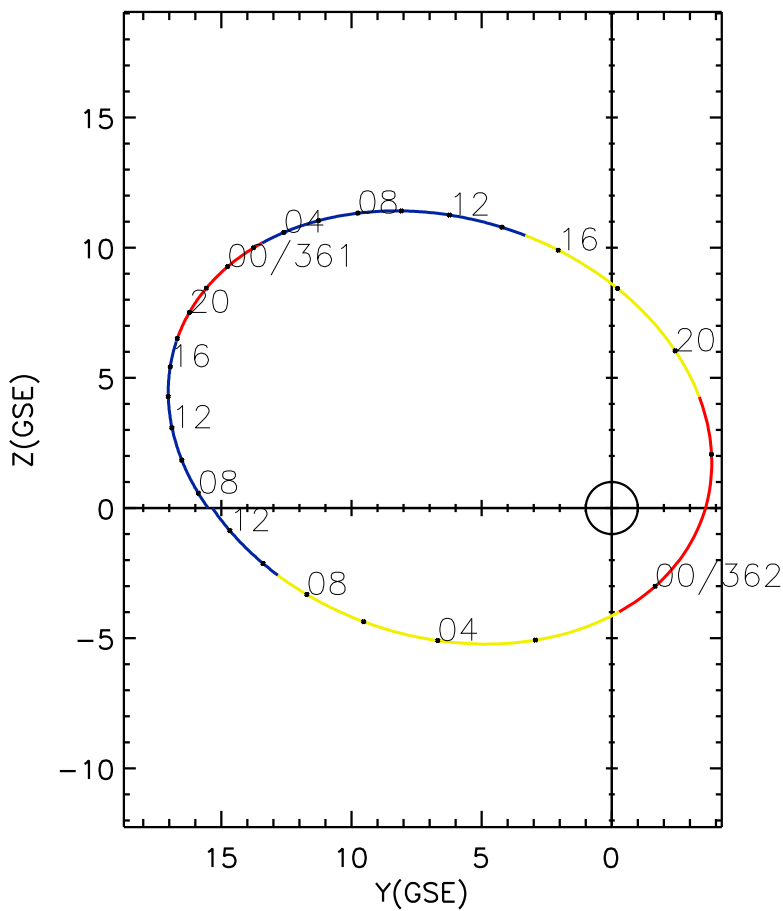
CLUSTER 2 orbit 2021 360 (12/26) 07:06 UT to 2021 362 (12/28) 13:21 UT
