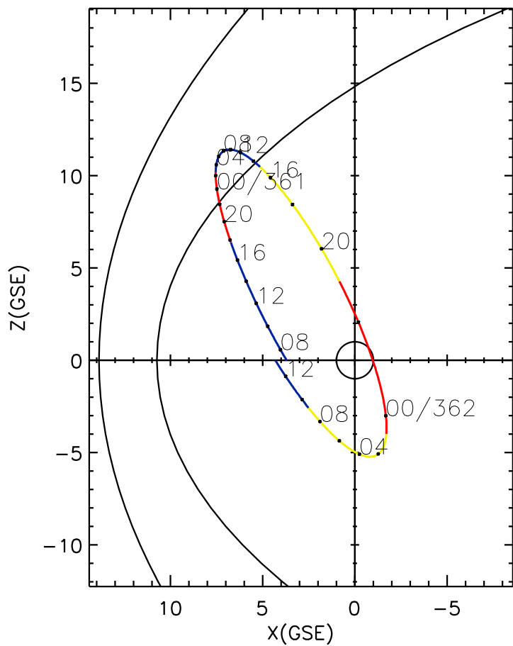
CLUSTER 2 orbit 2021 360 (12/26) 07:06 UT to 2021 362 (12/28) 13:21 UT
