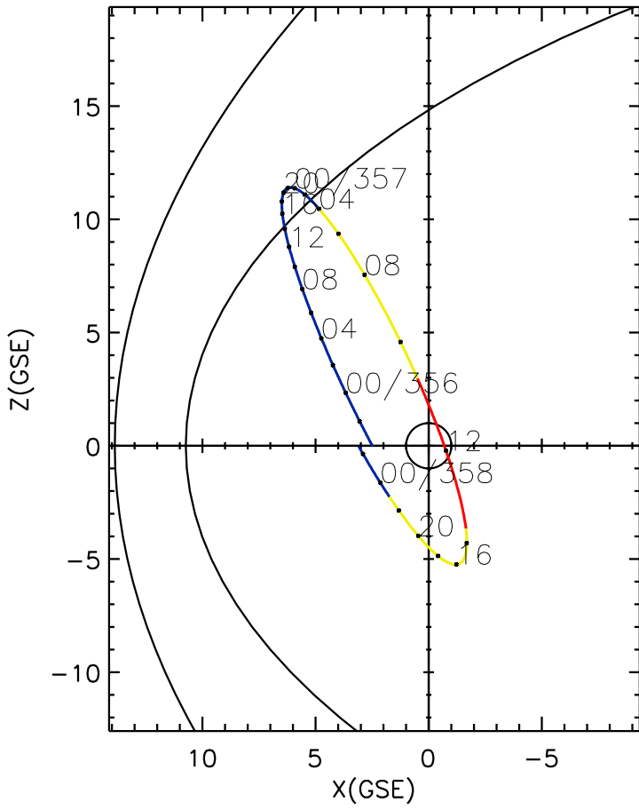
CLUSTER 2 orbit 2021 355 (12/21) 20:16 UT to 2021 358 (12/24) 02:31 UT
