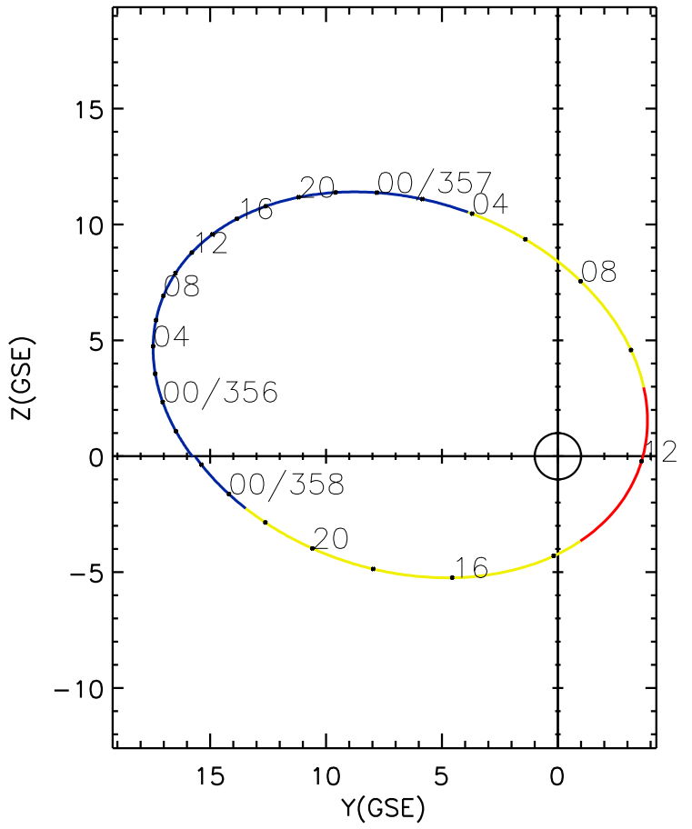
CLUSTER 2 orbit 2021 355 (12/21) 20:16 UT to 2021 358 (12/24) 02:31 UT
