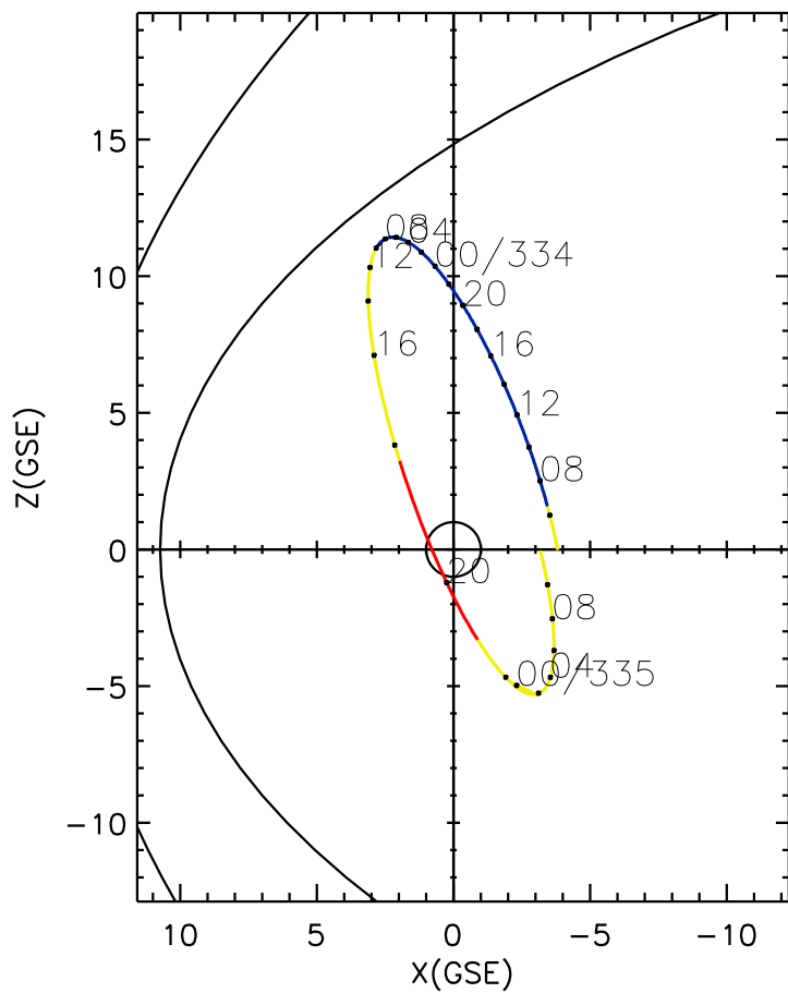
CLUSTER 2 orbit 2021 333 (11/29) 04:01 UT to 2021 335 (12/01) 11:56 UT
