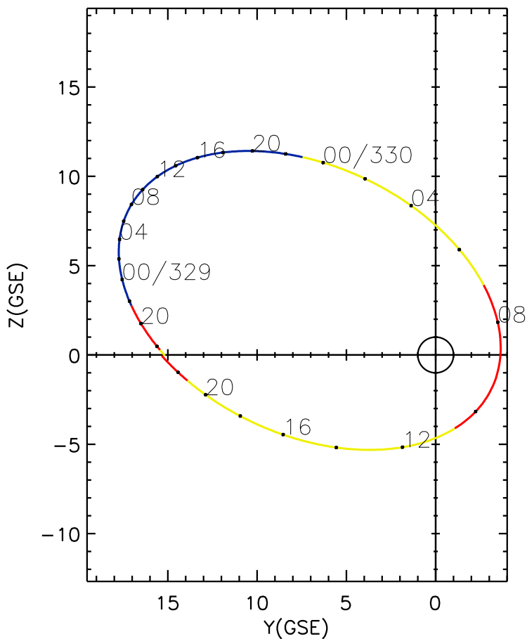
CLUSTER 2 orbit 2021 328 (11/24) 17:11 UT to 2021 330 (11/26) 23:26 UT
