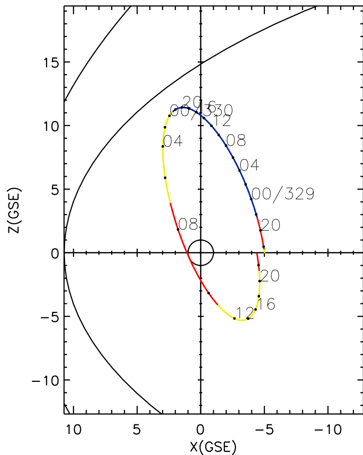
CLUSTER 2 orbit 2021 328 (11/24) 17:11 UT to 2021 330 (11/26) 23:26 UT
