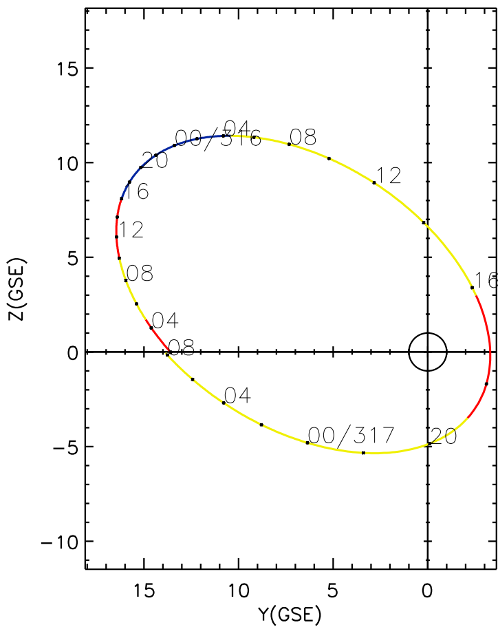
CLUSTER 2 orbit 2021 315 (11/11) 01:56 UT to 2021 317 (11/13) 08:11 UT
