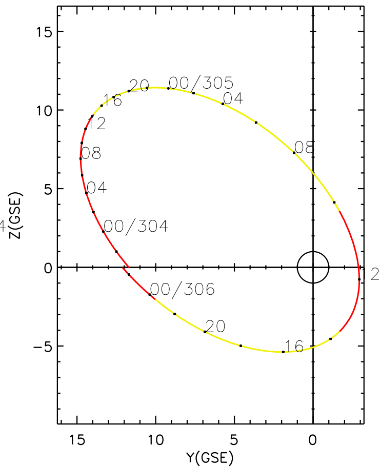
CLUSTER 2 orbit 2021 303 (10/30) 20:26 UT to 2021 306 (11/02) 02:41 UT
