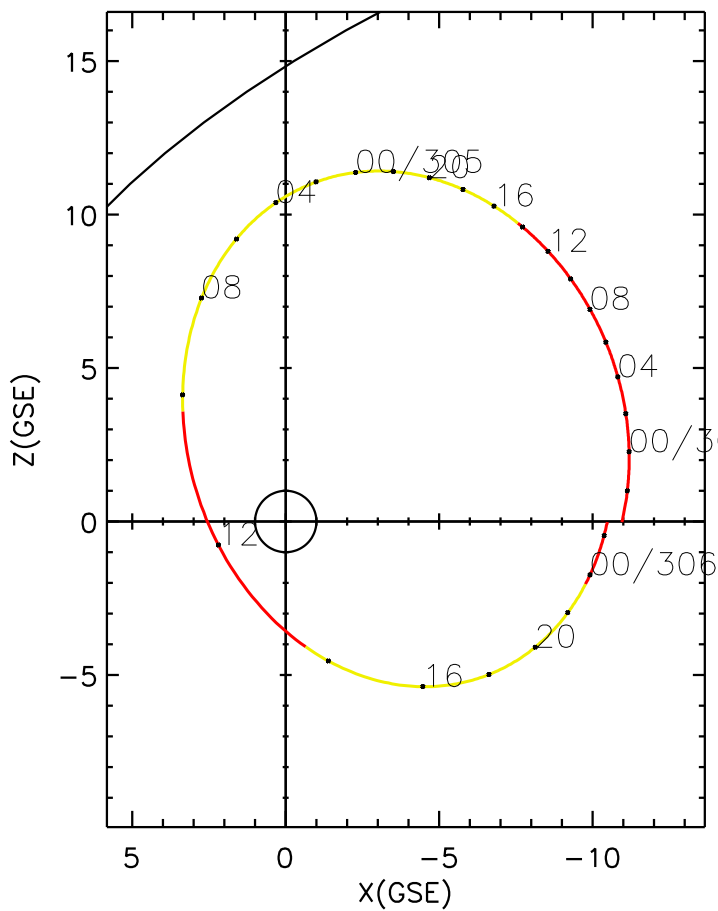
CLUSTER 2 orbit 2021 303 (10/30) 20:26 UT to 2021 306 (11/02) 02:41 UT
