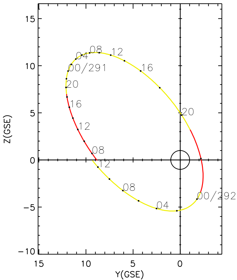
CLUSTER 2 orbit 2021 290 (10/17) 06:51 UT to 2021 292 (10/19) 13:06 UT
