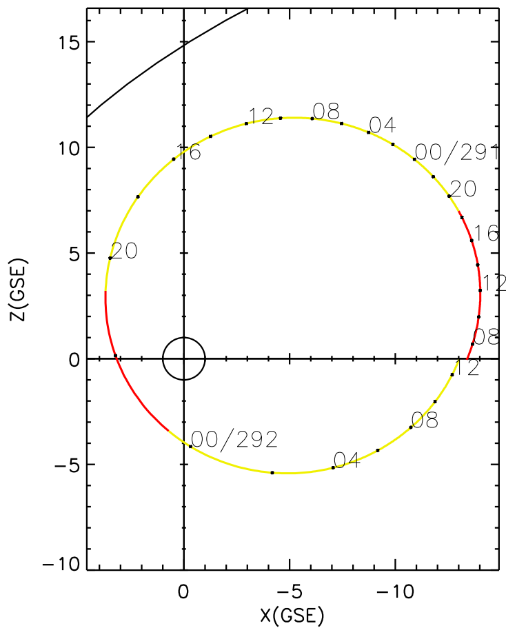
CLUSTER 2 orbit 2021 290 (10/17) 06:51 UT to 2021 292 (10/19) 13:06 UT
