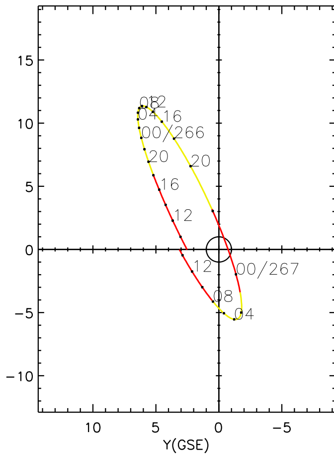
CLUSTER 2 orbit 2021 265 (09/22) 08:26 UT to 2021 267 (09/24) 14:41 UT
