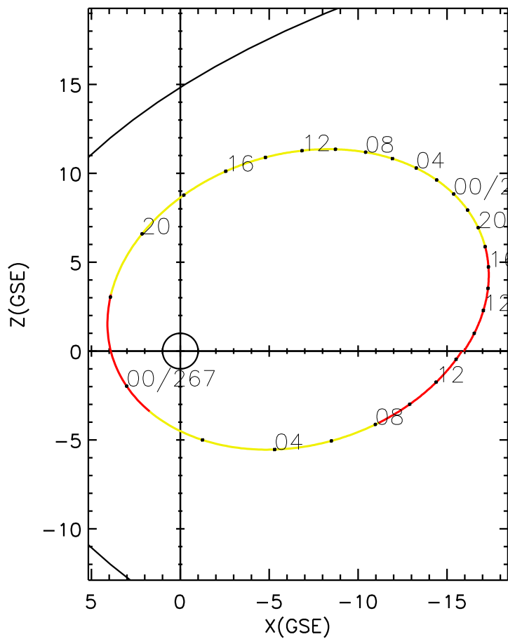
CLUSTER 2 orbit 2021 265 (09/22) 08:26 UT to 2021 267 (09/24) 14:41 UT
