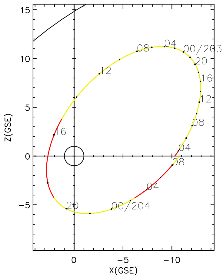
CLUSTER 2 orbit 2021 202 (07/21) 03:06 UT to 2021 204 (07/23) 09:21 UT
