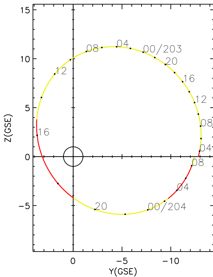
CLUSTER 2 orbit 2021 202 (07/21) 03:06 UT to 2021 204 (07/23) 09:21 UT
