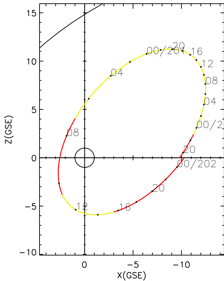
CLUSTER 2 orbit 2021 199 (07/18) 19:11 UT to 2021 202 (07/21) 01:26 UT
