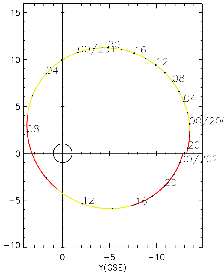
CLUSTER 2 orbit 2021 199 (07/18) 19:11 UT to 2021 202 (07/21) 01:26 UT
