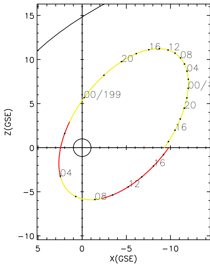
CLUSTER 2 orbit 2021 197 (07/16) 12:56 UT to 2021 199 (07/18) 19:11 UT
