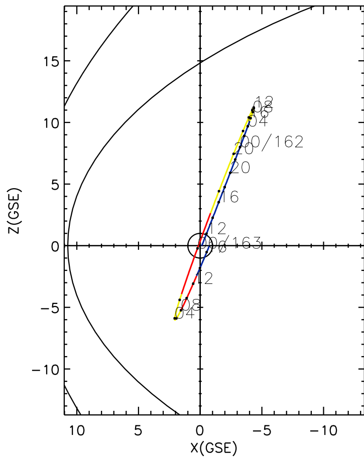
CLUSTER 2 orbit 2021 161 (06/10) 10:31 UT to 2021 163 (06/12) 16:46 UT
