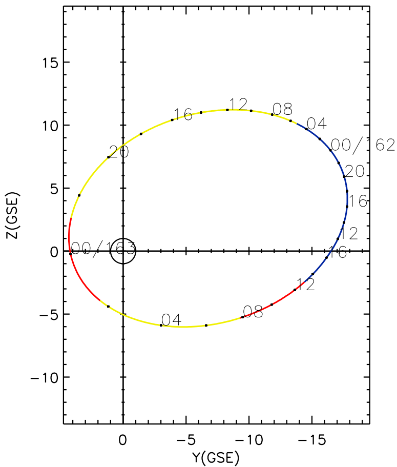
CLUSTER 2 orbit 2021 161 (06/10) 10:31 UT to 2021 163 (06/12) 16:46 UT
