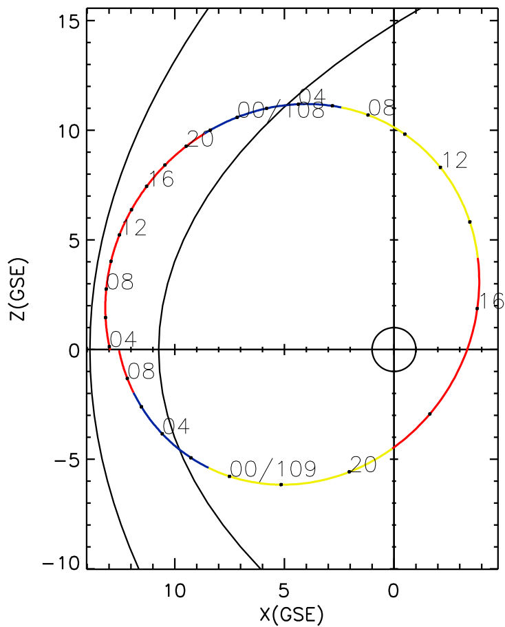
CLUSTER 2 orbit 2021 107 (04/17) 03:46 UT to 2021 109 (04/19) 09:56 UT
