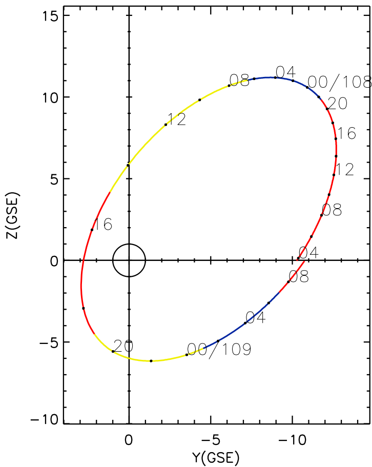
CLUSTER 2 orbit 2021 107 (04/17) 03:46 UT to 2021 109 (04/19) 09:56 UT
