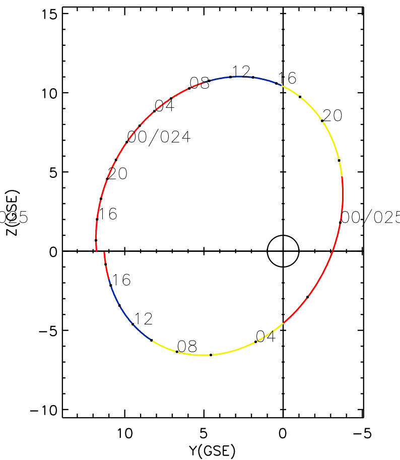
CLUSTER 2 orbit 2021 023 (01/23) 12:56 UT to 2021 025 (01/25) 19:11 UT
