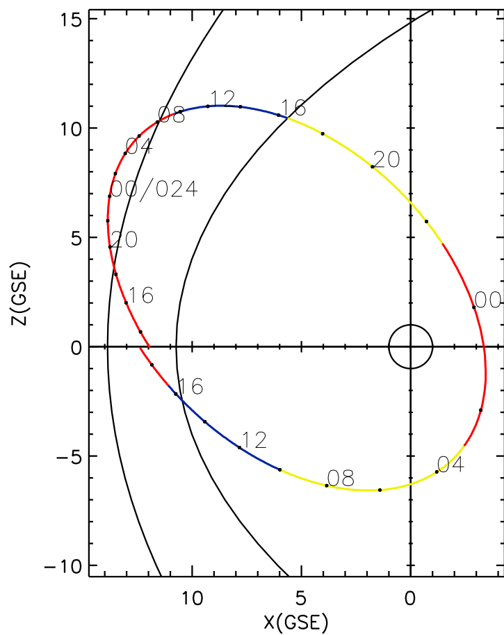
CLUSTER 2 orbit 2021 023 (01/23) 12:56 UT to 2021 025 (01/25) 19:11 UT
