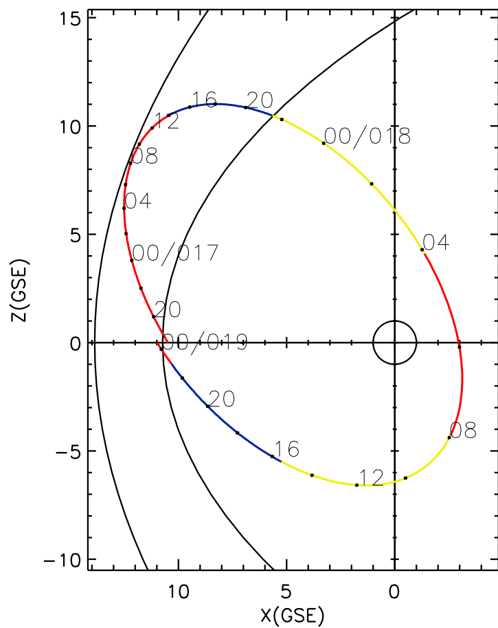
CLUSTER 2 orbit 2021 016 (01/16) 18:11 UT to 2021 019 (01/19) 00:26 UT
