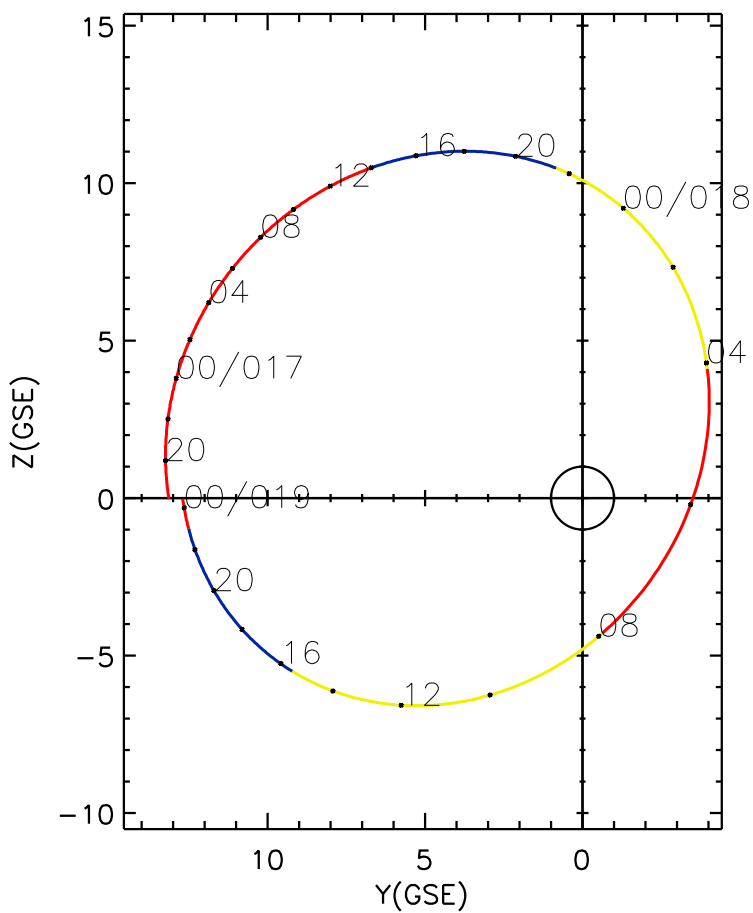
CLUSTER 2 orbit 2021 016 (01/16) 18:11 UT to 2021 019 (01/19) 00:26 UT
