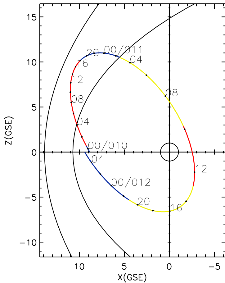
CLUSTER 2 orbit 2021 009 (01/09) 23:26 UT to 2021 012 (01/12) 05:41 UT
