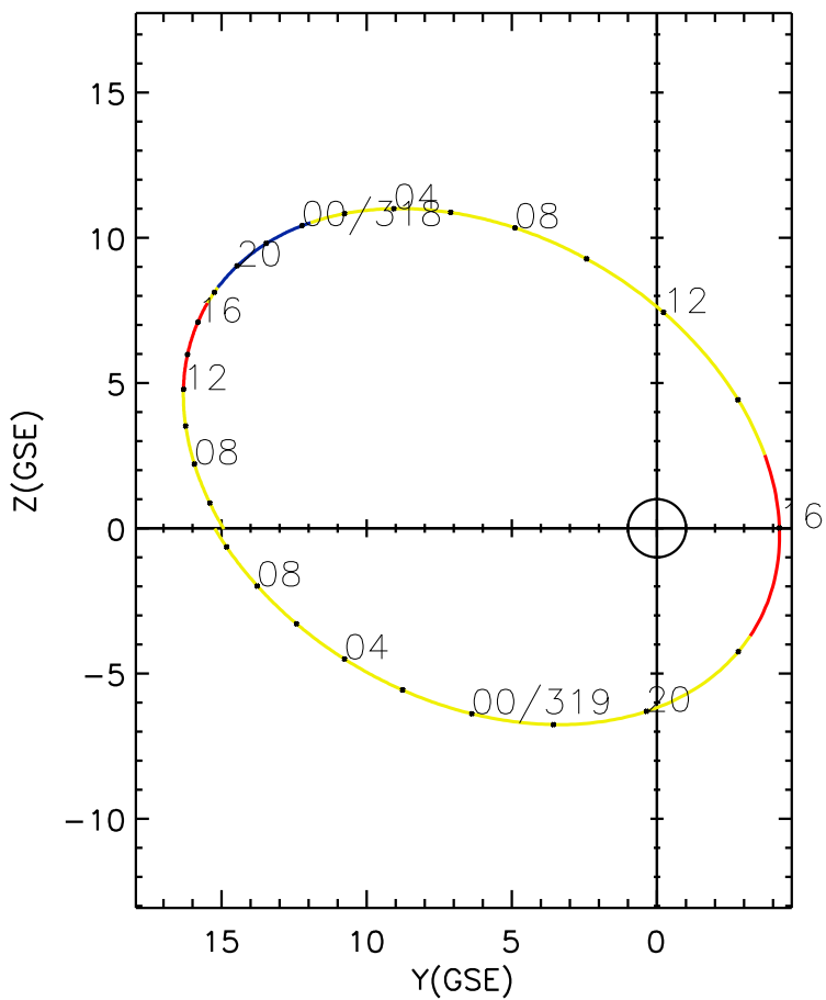
CLUSTER 2 orbit 2020 317 (11/12) 04:41 UT to 2020 319 (11/14) 10:56 UT
