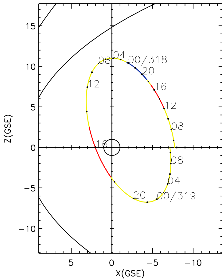
CLUSTER 2 orbit 2020 317 (11/12) 04:41 UT to 2020 319 (11/14) 10:56 UT
