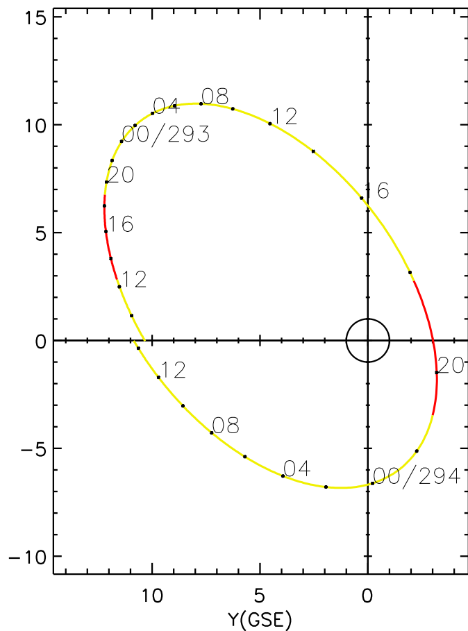
CLUSTER 2 orbit 2020 292 (10/18) 08:16 UT to 2020 294 (10/20) 14:31 UT
