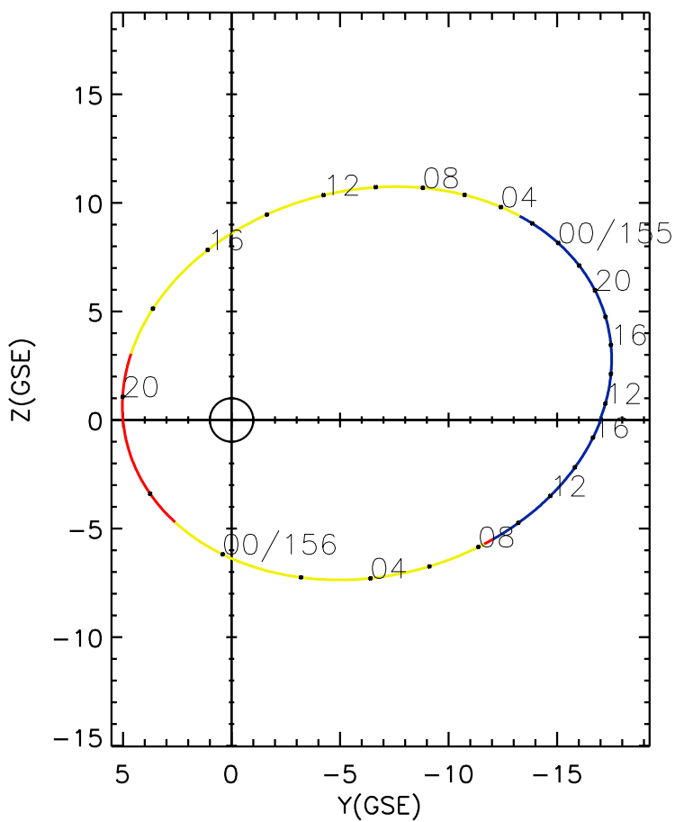
CLUSTER 2 orbit 2020 154 (06/02) 10:51 UT to 2020 156 (06/04) 17:06 UT
