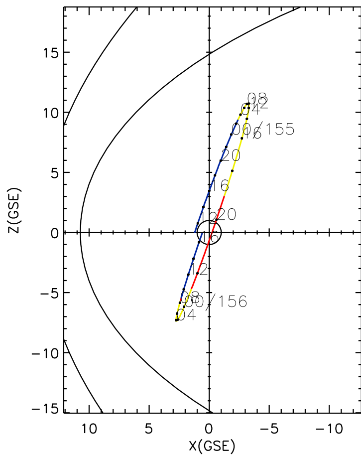
CLUSTER 2 orbit 2020 154 (06/02) 10:51 UT to 2020 156 (06/04) 17:06 UT
