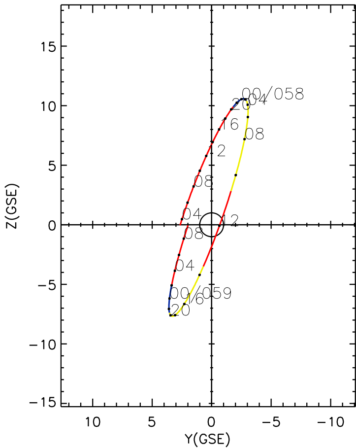
CLUSTER 2 orbit 2020 057 (02/26) 03:16 UT to 2020 059 (02/28) 09:36 UT
