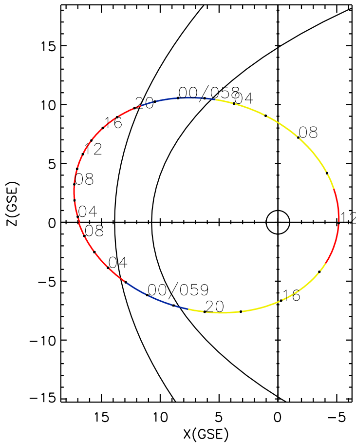
CLUSTER 2 orbit 2020 057 (02/26) 03:16 UT to 2020 059 (02/28) 09:36 UT
