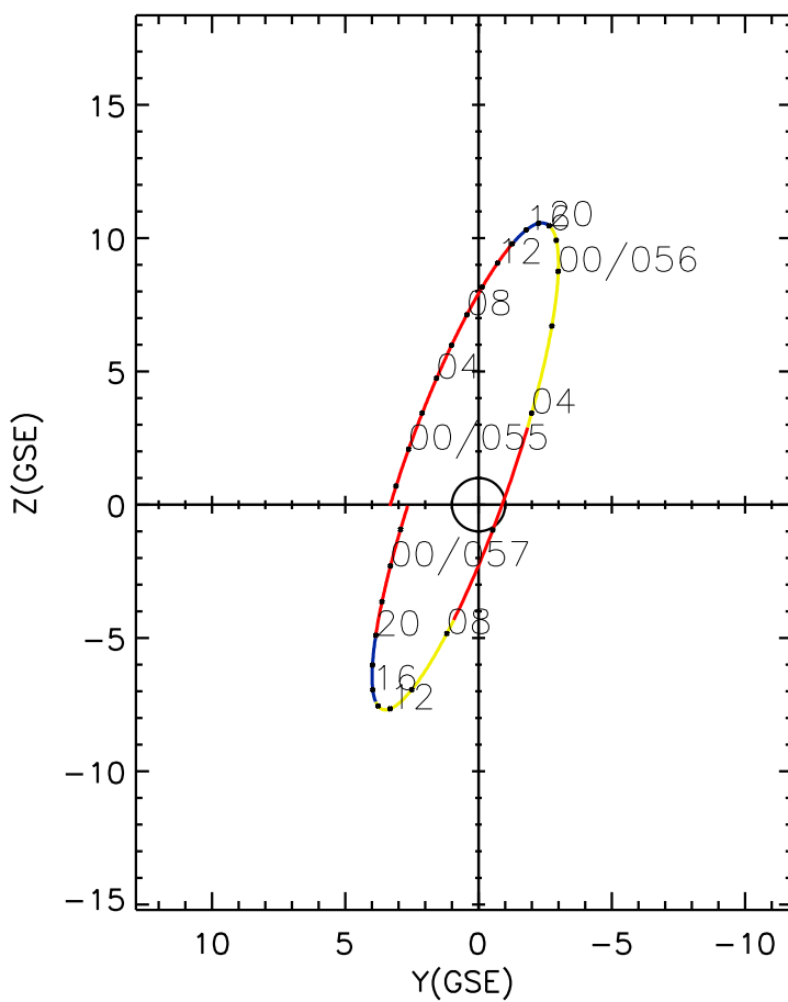
CLUSTER 2 orbit 2020 054 (02/23) 20:56 UT to 2020 057 (02/26) 03:16 UT
