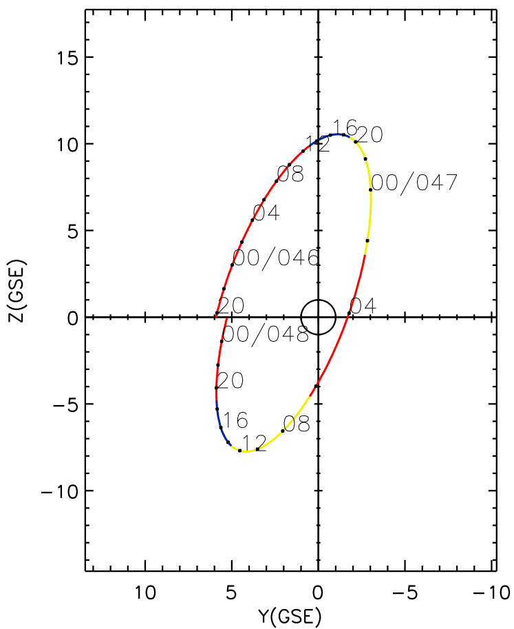
CLUSTER 2 orbit 2020 045 (02/14) 19:36 UT to 2020 048 (02/17) 01:56 UT
