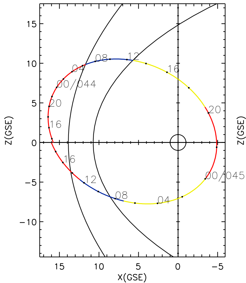
CLUSTER 2 orbit 2020 043 (02/12) 13:16 UT to 2020 045 (02/14) 19:36 UT
