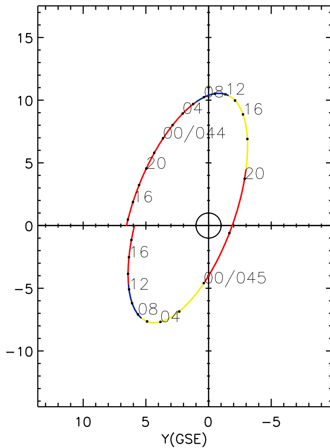
CLUSTER 2 orbit 2020 043 (02/12) 13:16 UT to 2020 045 (02/14) 19:36 UT
