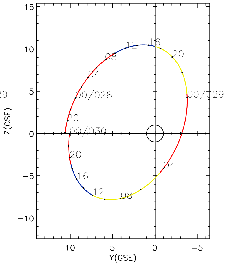
CLUSTER 2 orbit 2020 027 (01/27) 17:51 UT to 2020 030 (01/30) 00:06 UT
