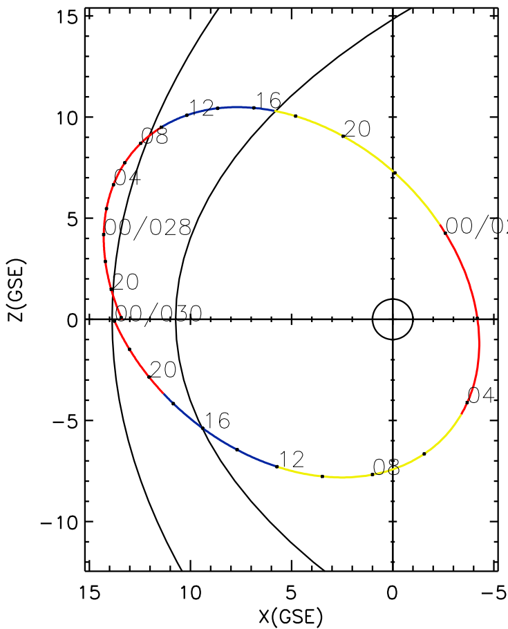
CLUSTER 2 orbit 2020 027 (01/27) 17:51 UT to 2020 030 (01/30) 00:06 UT
