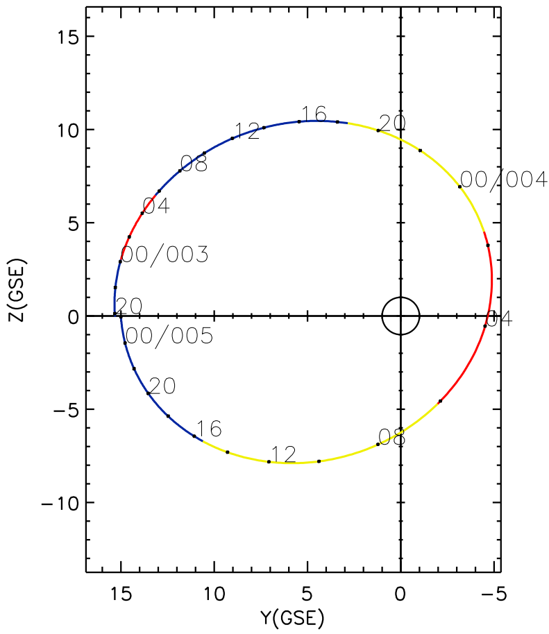
CLUSTER 2 orbit 2020 002 (01/02) 19:46 UT to 2020 005 (01/05) 02:01 UT
