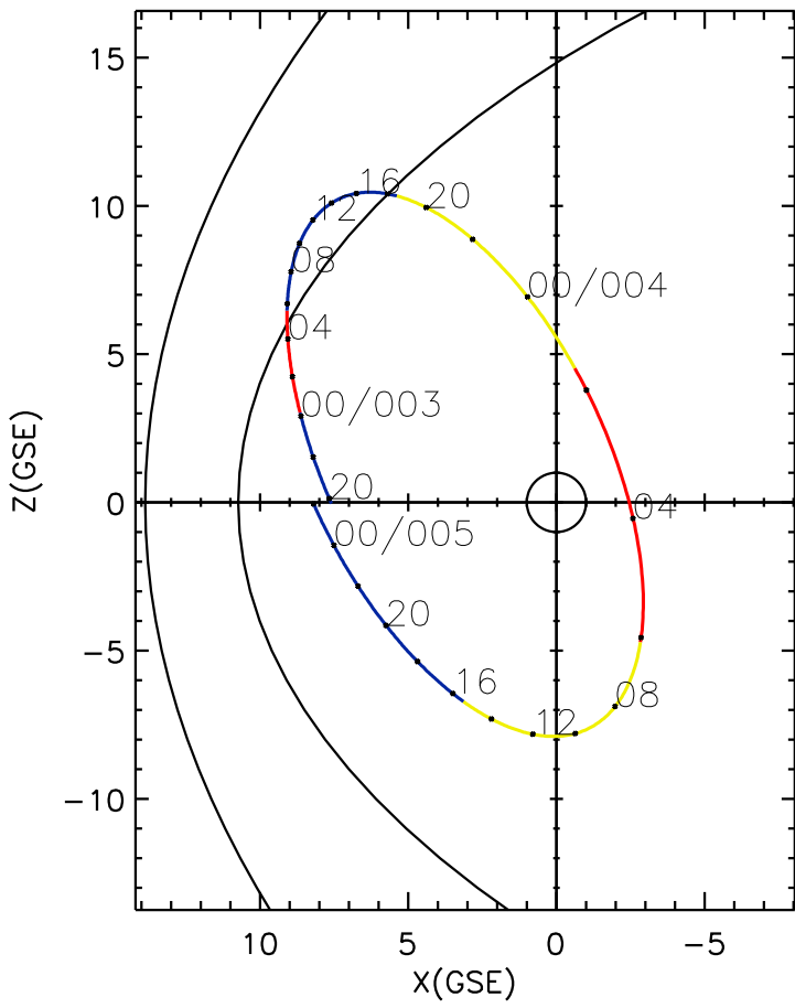
CLUSTER 2 orbit 2020 002 (01/02) 19:46 UT to 2020 005 (01/05) 02:01 UT
