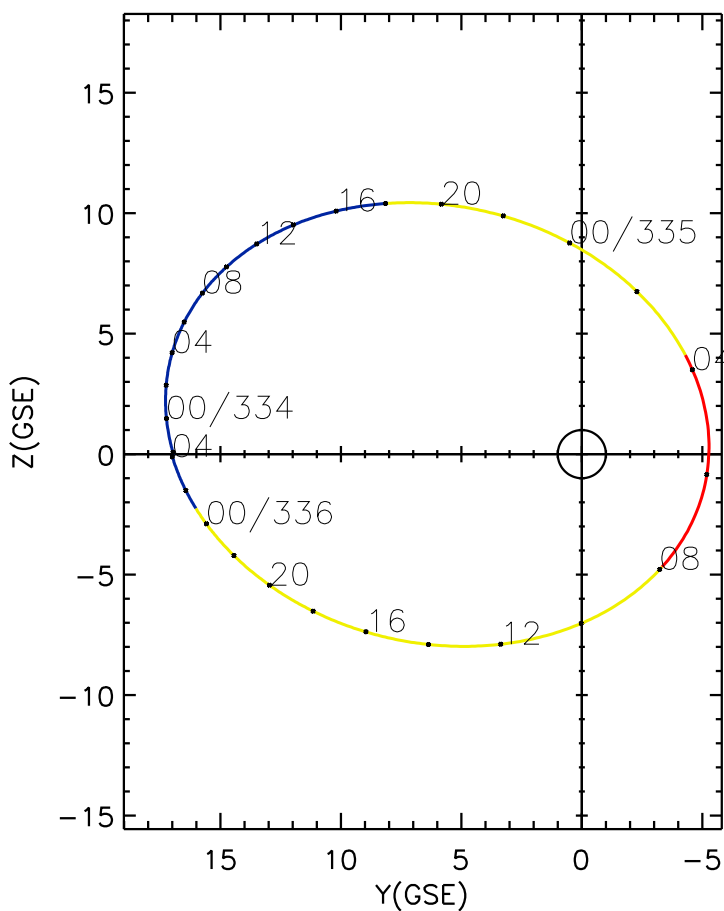
CLUSTER 2 orbit 2019 333 (11/29) 21:51 UT to 2019 336 (12/02) 04:06 UT
