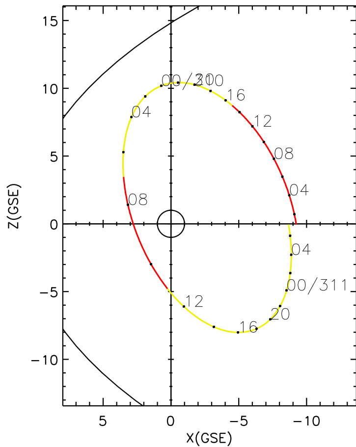
CLUSTER 2 orbit 2019 309 (11/05) 00:56 UT to 2019 311 (11/07) 07:11 UT
