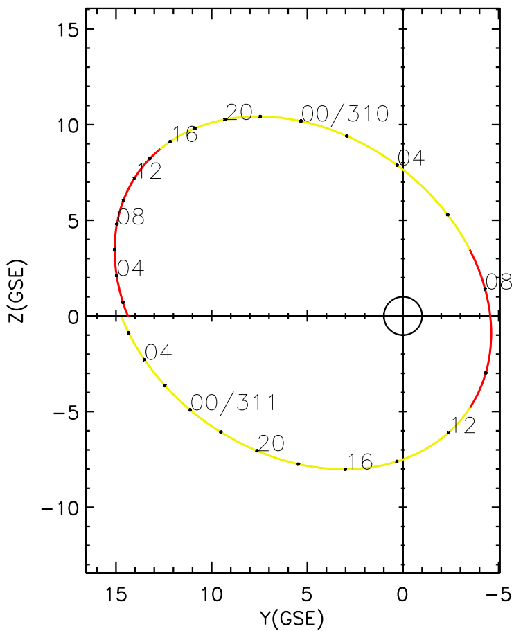
CLUSTER 2 orbit 2019 309 (11/05) 00:56 UT to 2019 311 (11/07) 07:11 UT
