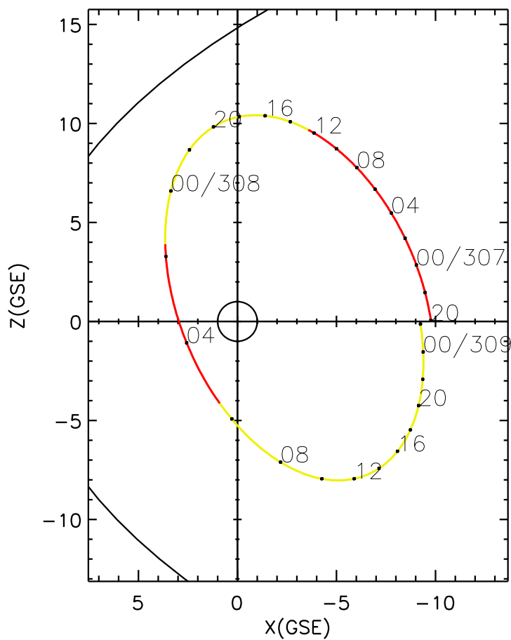
CLUSTER 2 orbit 2019 306 (11/02) 19:51 UT to 2019 309 (11/05) 02:06 UT
