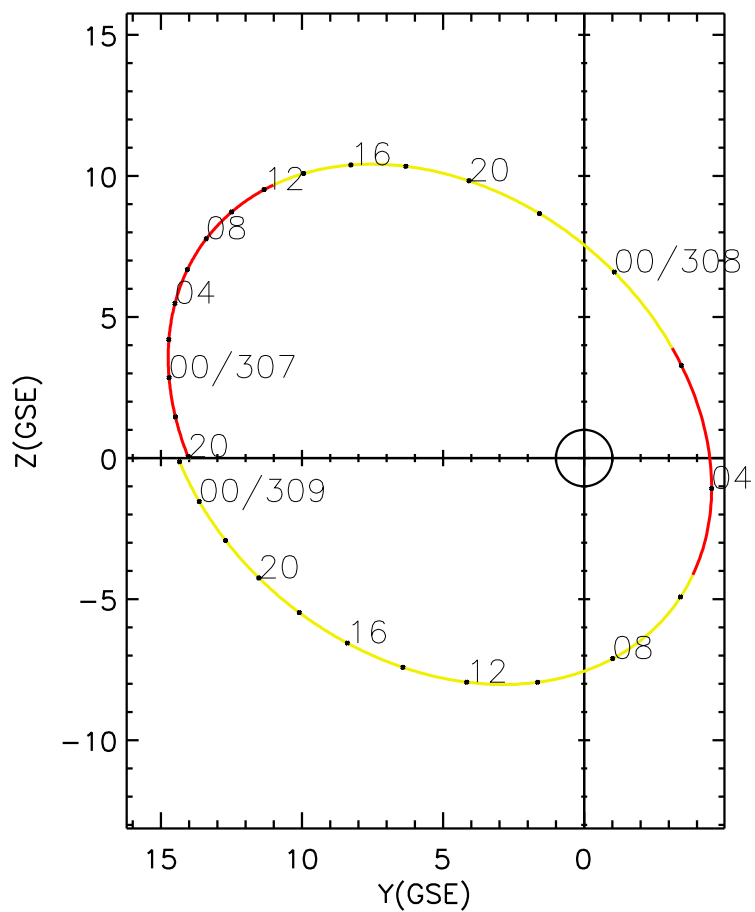
CLUSTER 2 orbit 2019 306 (11/02) 19:51 UT to 2019 309 (11/05) 02:06 UT
