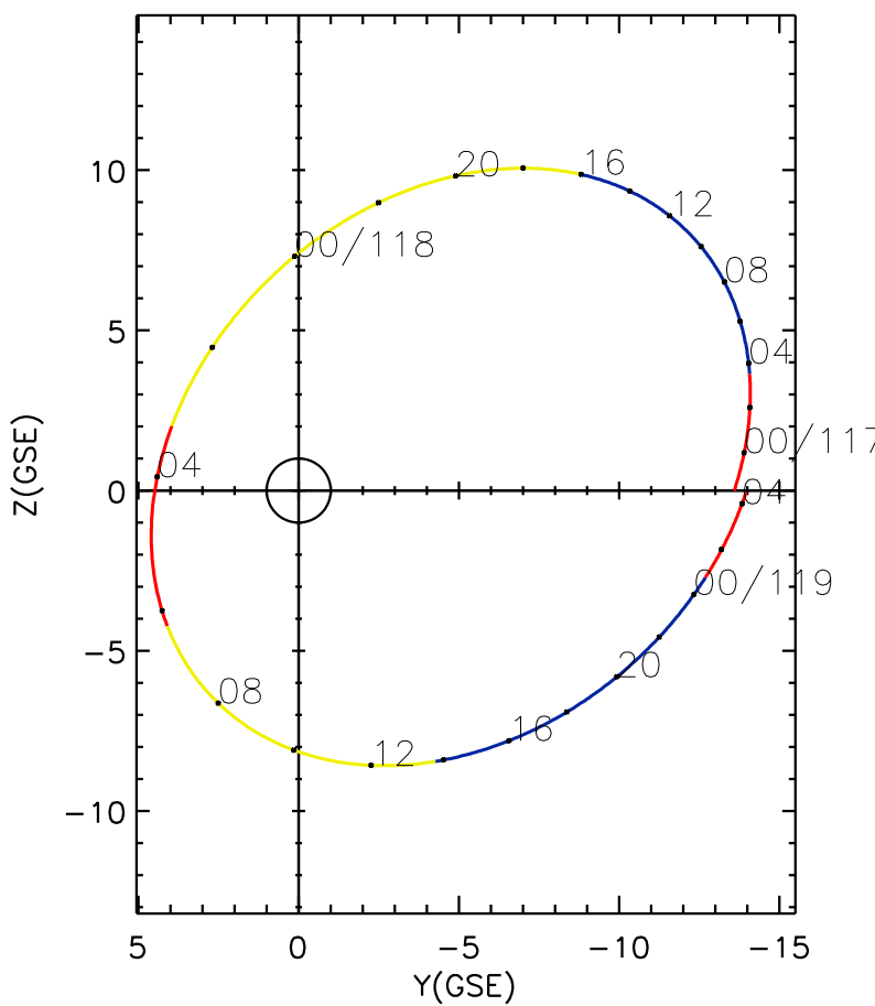
CLUSTER 2 orbit 2019 116 (04/26) 22:21 UT to 2019 119 (04/29) 04:31 UT
