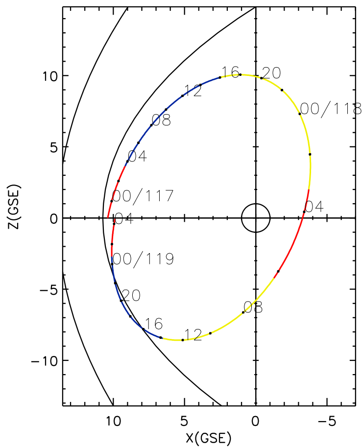
CLUSTER 2 orbit 2019 116 (04/26) 22:21 UT to 2019 119 (04/29) 04:31 UT
