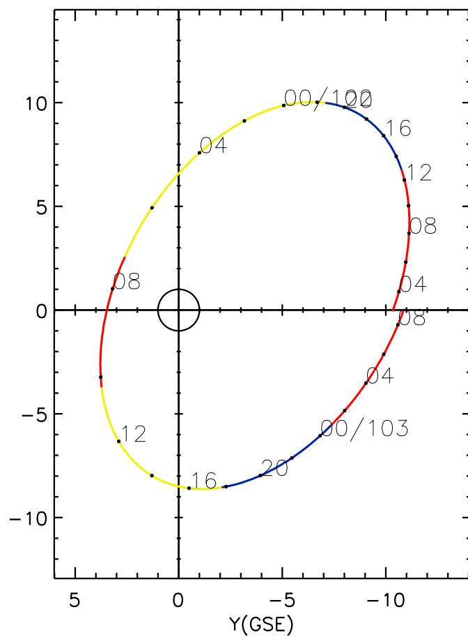
CLUSTER 2 orbit 2019 101 (04/11) 02:41 UT to 2019 103 (04/13) 08:56 UT
