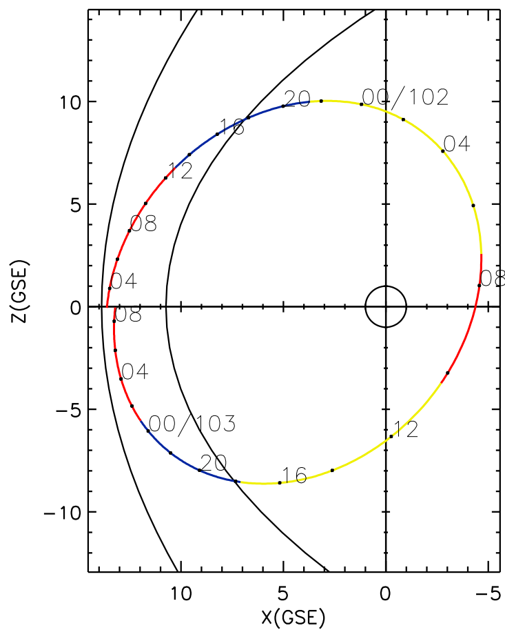
CLUSTER 2 orbit 2019 101 (04/11) 02:41 UT to 2019 103 (04/13) 08:56 UT
