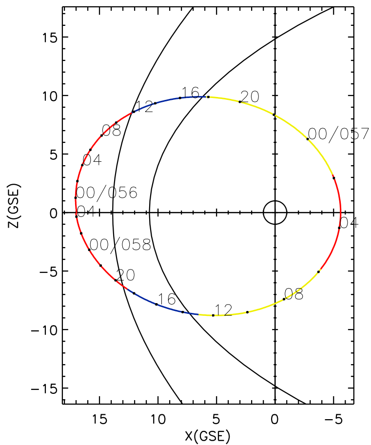
CLUSTER 2 orbit 2019 055 (02/24) 22:11 UT to 2019 058 (02/27) 04:26 UT
