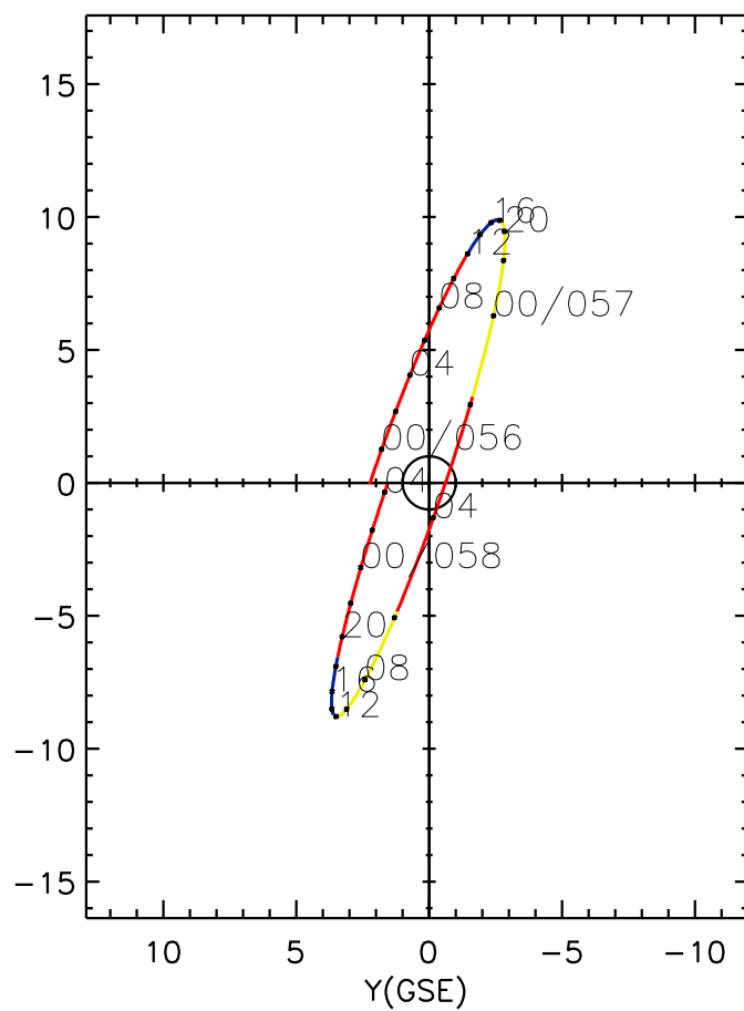
CLUSTER 2 orbit 2019 055 (02/24) 22:11 UT to 2019 058 (02/27) 04:26 UT
