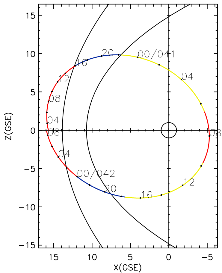
CLUSTER 2 orbit 2019 040 (02/09) 02:41 UT to 2019 042 (02/11) 08:51 UT
