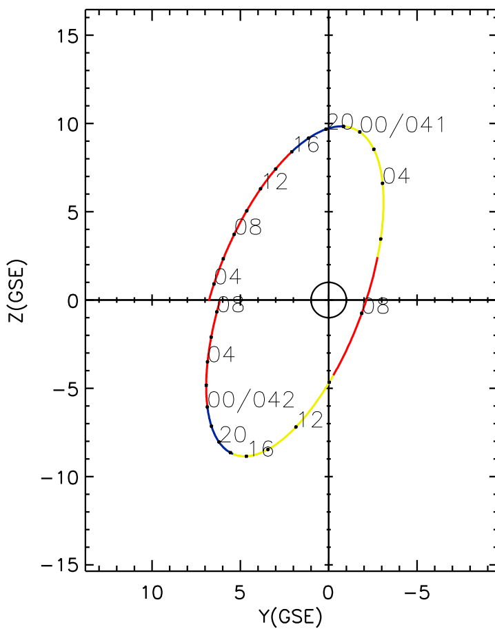
CLUSTER 2 orbit 2019 040 (02/09) 02:41 UT to 2019 042 (02/11) 08:51 UT
