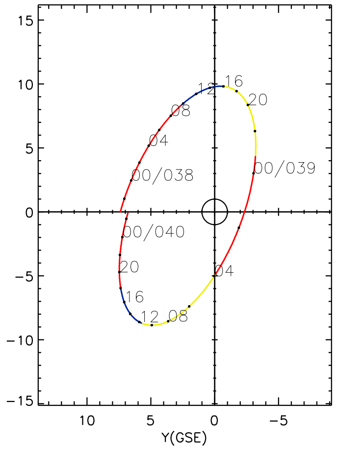
CLUSTER 2 orbit 2019 037 (02/06) 20:31 UT to 2019 040 (02/09) 02:41 UT
