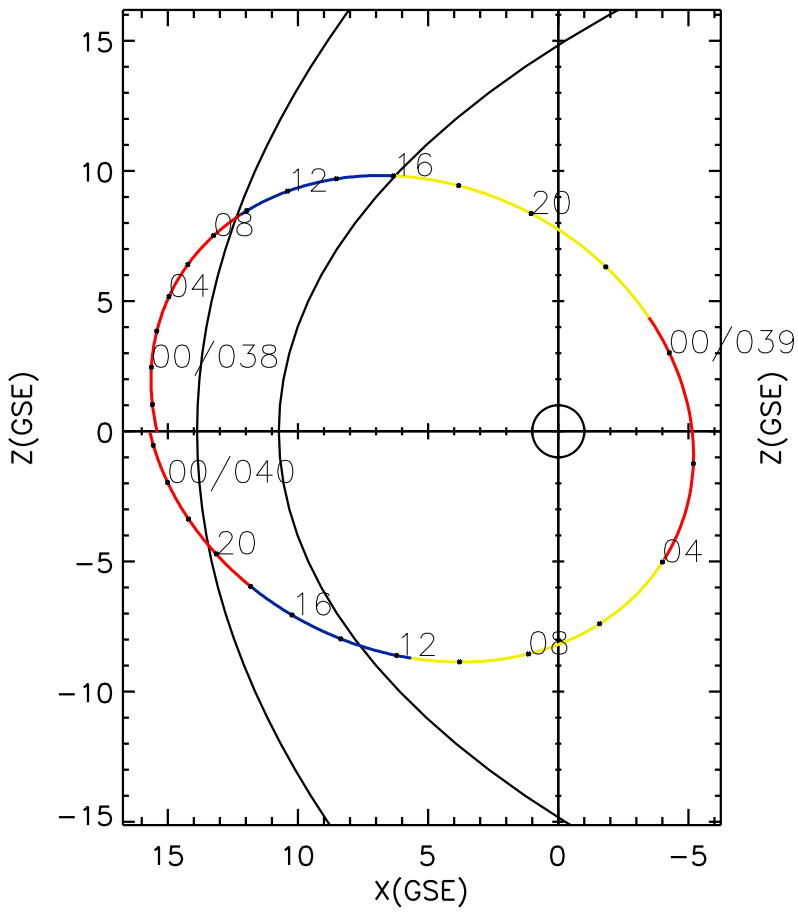
CLUSTER 2 orbit 2019 037 (02/06) 20:31 UT to 2019 040 (02/09) 02:41 UT
