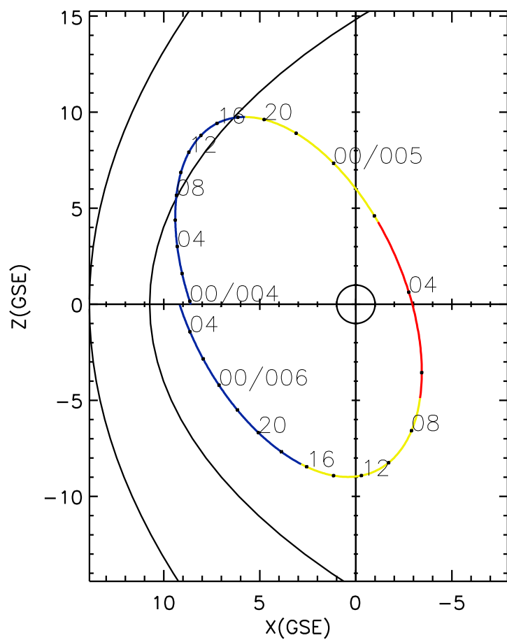
CLUSTER 2 orbit 2019 003 (01/03) 23:46 UT to 2019 006 (01/06) 05:56 UT
