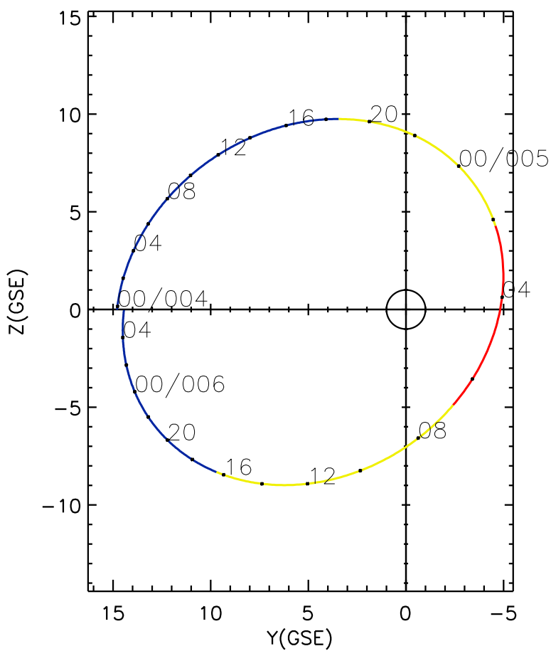
CLUSTER 2 orbit 2019 003 (01/03) 23:46 UT to 2019 006 (01/06) 05:56 UT
