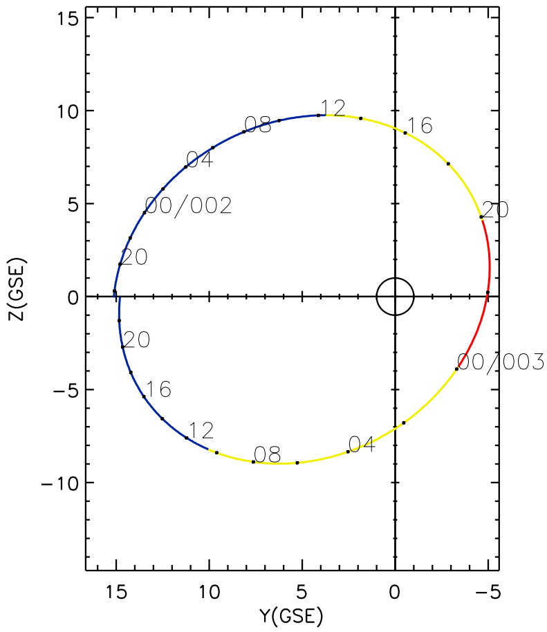
CLUSTER 2 orbit 2019 001 (01/01) 17:31 UT to 2019 003 (01/03) 23:46 UT
