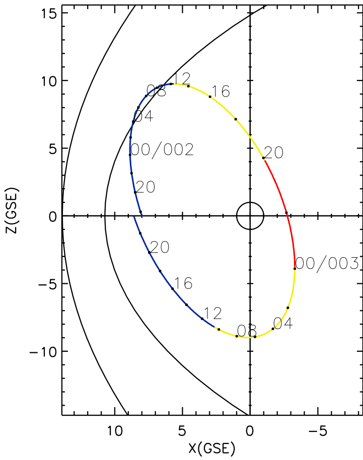
CLUSTER 2 orbit 2019 001 (01/01) 17:31 UT to 2019 003 (01/03) 23:46 UT
