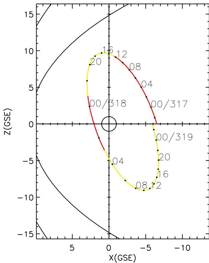
CLUSTER 2 orbit 2018 316 (11/12) 20:46 UT to 2018 319 (11/15) 03:01 UT
