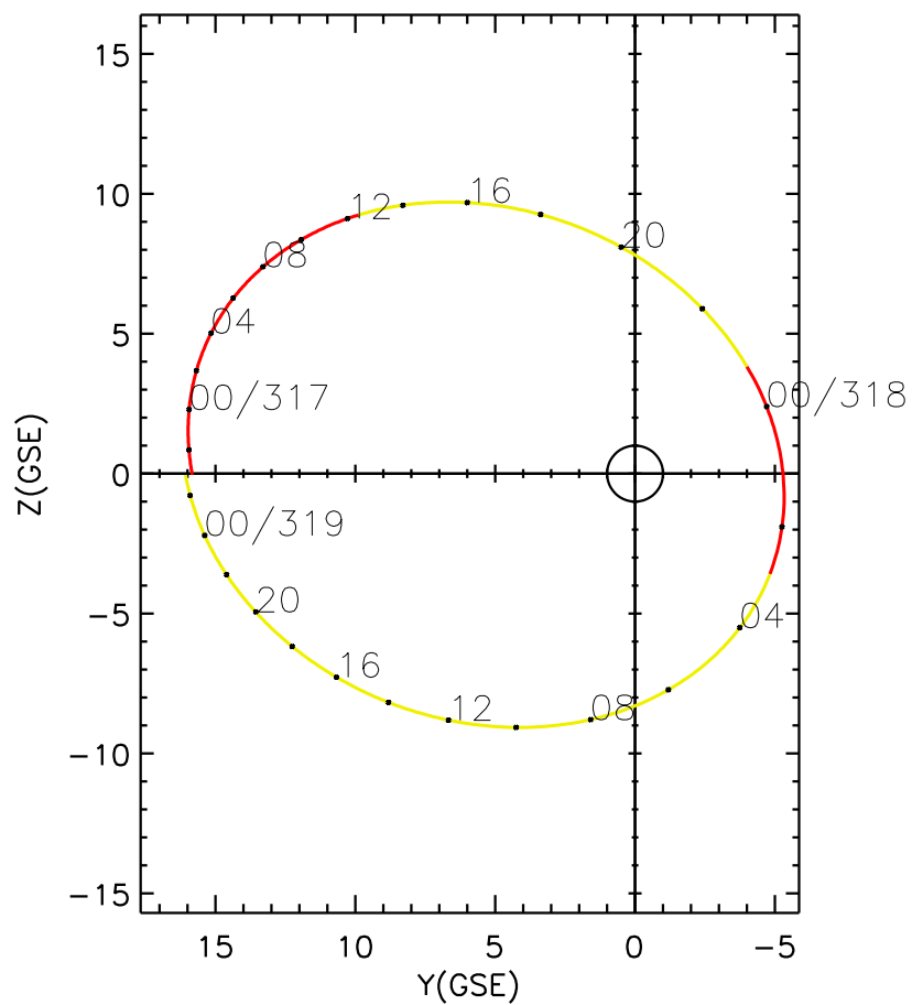
CLUSTER 2 orbit 2018 316 (11/12) 20:46 UT to 2018 319 (11/15) 03:01 UT
