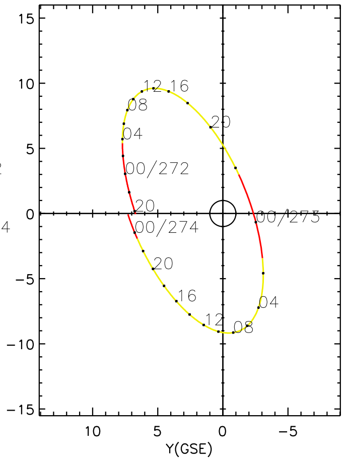
CLUSTER 2 orbit 2018 271 (09/28) 19:41 UT to 2018 274 (10/01) 01:56 UT
