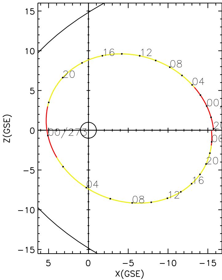
CLUSTER 2 orbit 2018 271 (09/28) 19:41 UT to 2018 274 (10/01) 01:56 UT
