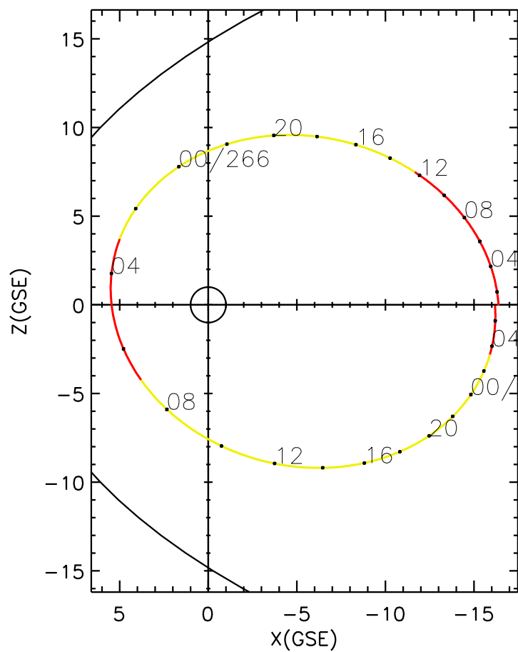
CLUSTER 2 orbit 2018 265 (09/22) 00:56 UT to 2018 267 (09/24) 07:11 UT
