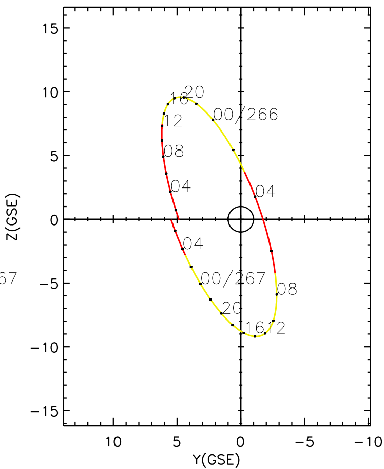
CLUSTER 2 orbit 2018 265 (09/22) 00:56 UT to 2018 267 (09/24) 07:11 UT
