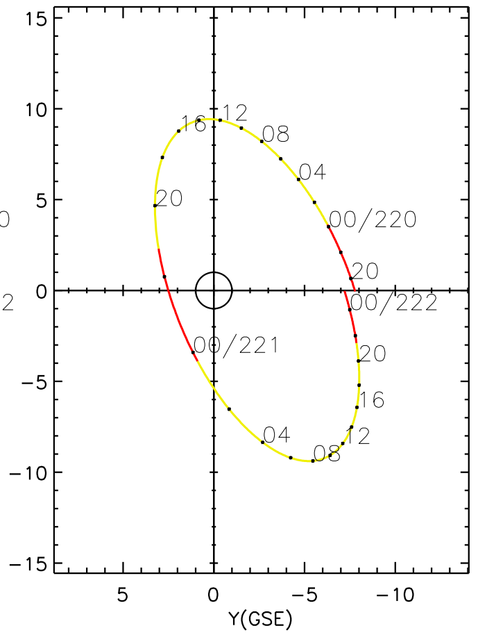
CLUSTER 2 orbit 2018 219 (08/07) 19:01 UT to 2018 222 (08/10) 01:26 UT
