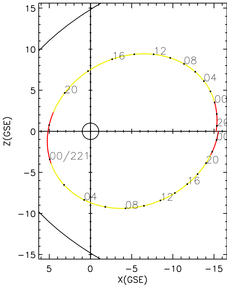
CLUSTER 2 orbit 2018 219 (08/07) 19:01 UT to 2018 222 (08/10) 01:26 UT
