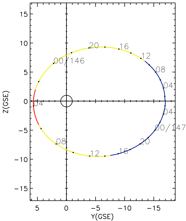
CLUSTER 2 orbit 2018 145 (05/25) 00:51 UT to 2018 147 (05/27) 07:06 UT
