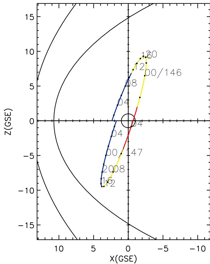
CLUSTER 2 orbit 2018 145 (05/25) 00:51 UT to 2018 147 (05/27) 07:06 UT
