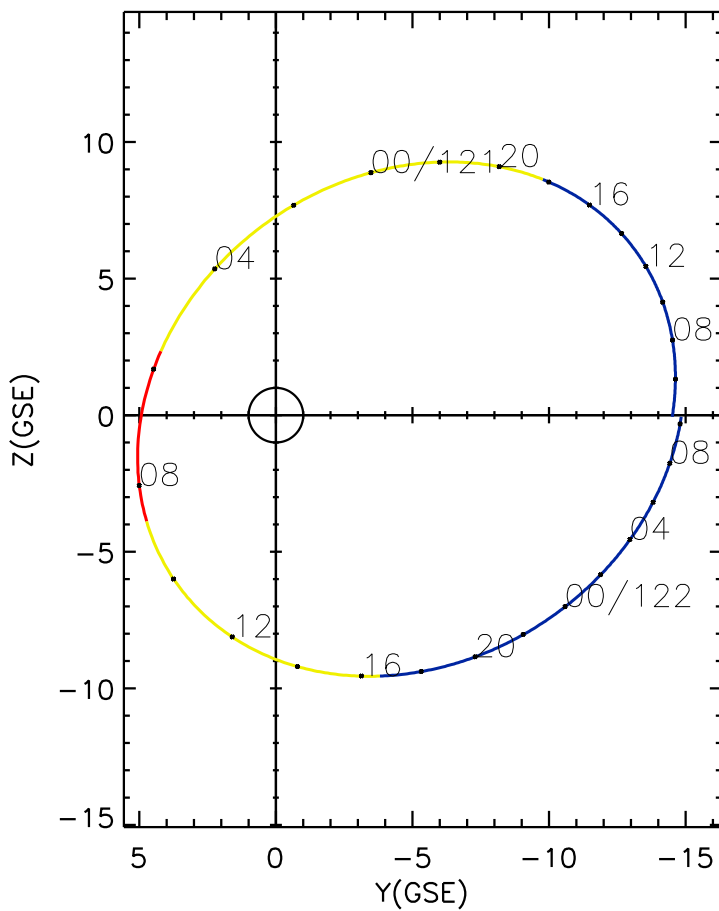
CLUSTER 2 orbit 2018 120 (04/30) 04:06 UT to 2018 122 (05/02) 10:21 UT
