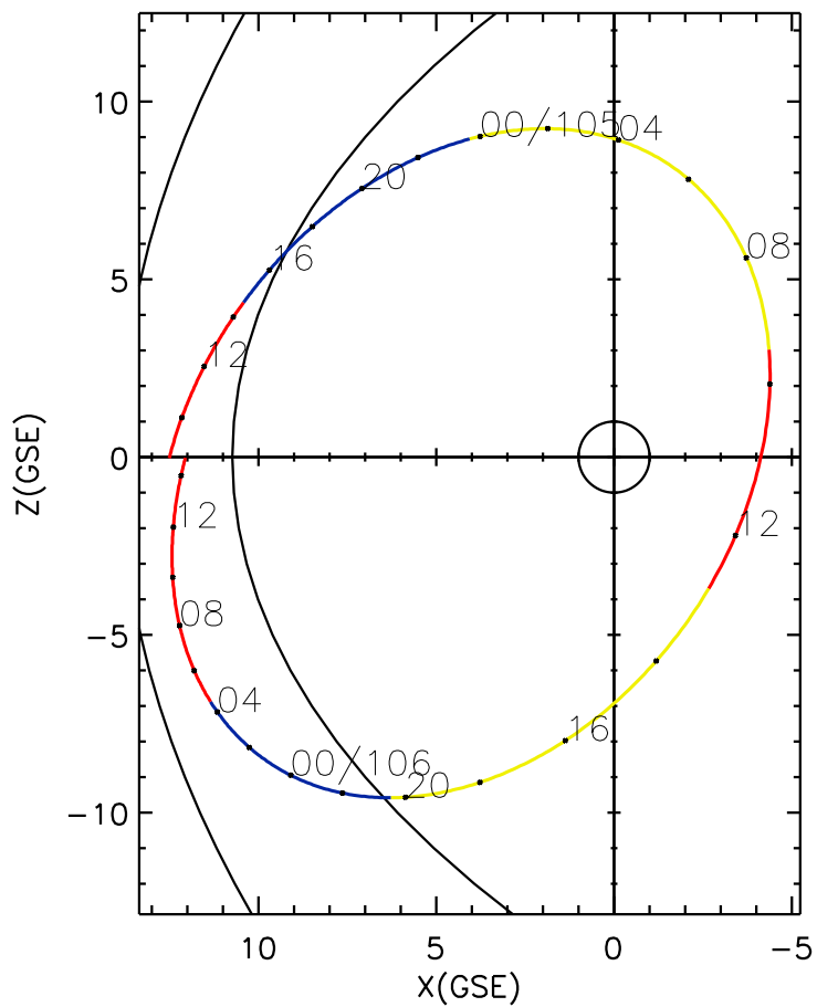
CLUSTER 2 orbit 2018 104 (04/14) 08:26 UT to 2018 106 (04/16) 14:41 UT
