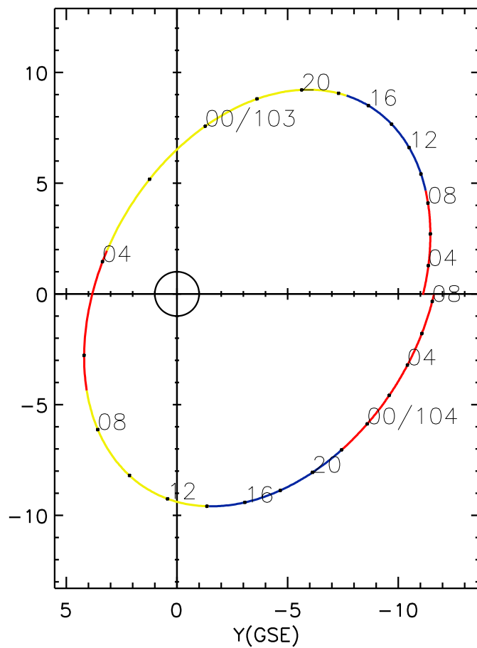
CLUSTER 2 orbit 2018 102 (04/12) 02:11 UT to 2018 104 (04/14) 08:26 UT
