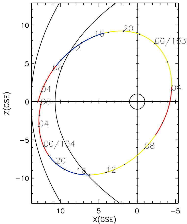
CLUSTER 2 orbit 2018 102 (04/12) 02:11 UT to 2018 104 (04/14) 08:26 UT
