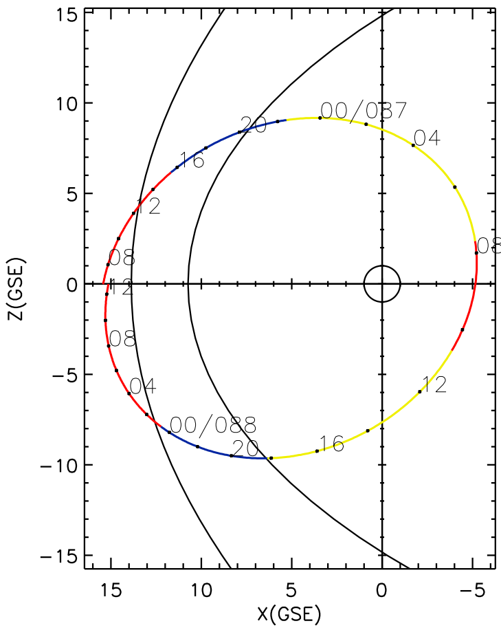
CLUSTER 2 orbit 2018 086 (03/27) 06:31 UT to 2018 088 (03/29) 12:46 UT
