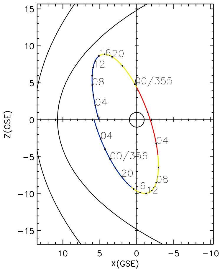
CLUSTER 2 orbit 2017 354 (12/20) 01:16 UT to 2017 356 (12/22) 07:31 UT
