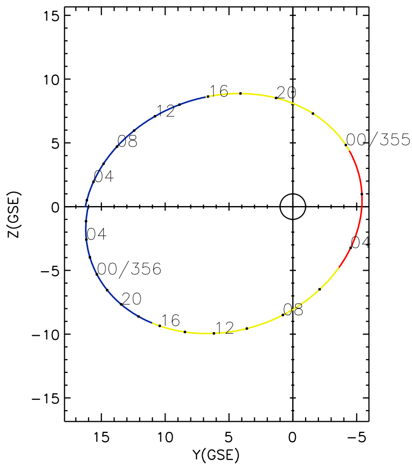
CLUSTER 2 orbit 2017 354 (12/20) 01:16 UT to 2017 356 (12/22) 07:31 UT
