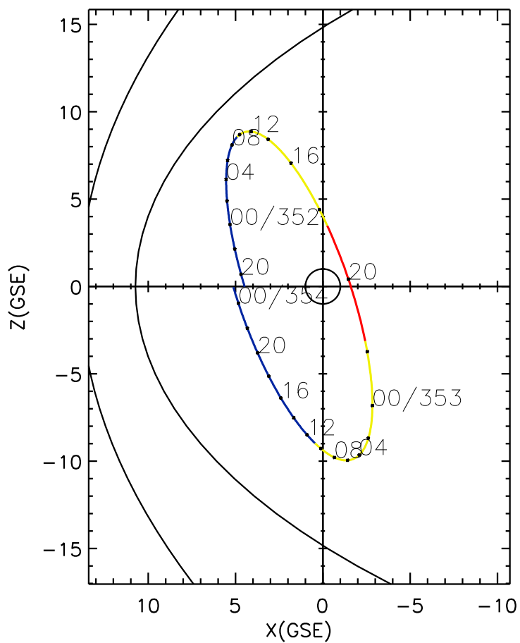
CLUSTER 2 orbit 2017 351 (12/17) 19:01 UT to 2017 354 (12/20) 01:16 UT
