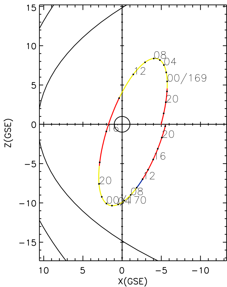
CLUSTER 2 orbit 2017 168 (06/17) 16:01 UT to 2017 170 (06/19) 22:16 UT
