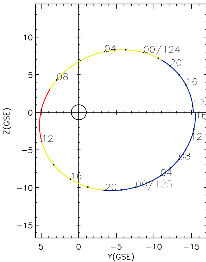
CLUSTER 2 orbit 2017 123 (05/03) 10:51 UT to 2017 125 (05/05) 17:06 UT
