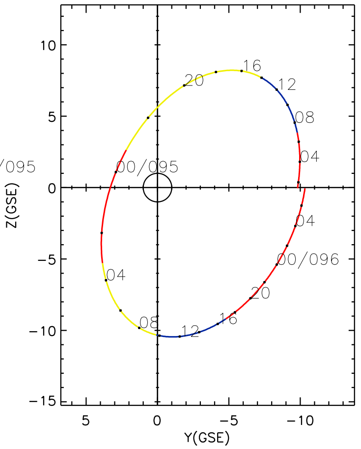
CLUSTER 2 orbit 2017 094 (04/04) 01:26 UT to 2017 096 (04/06) 07:41 UT
