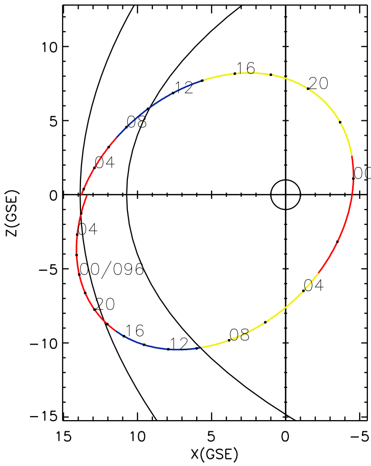
CLUSTER 2 orbit 2017 094 (04/04) 01:26 UT to 2017 096 (04/06) 07:41 UT
